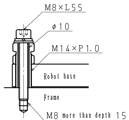
Details of the adjuster (S=1:2)
